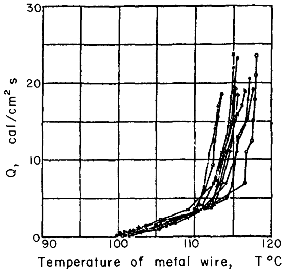
FIG. 5. Nickel wire, d = 0.14 mm; water temperature = 100^{\circ}\text{C} .
