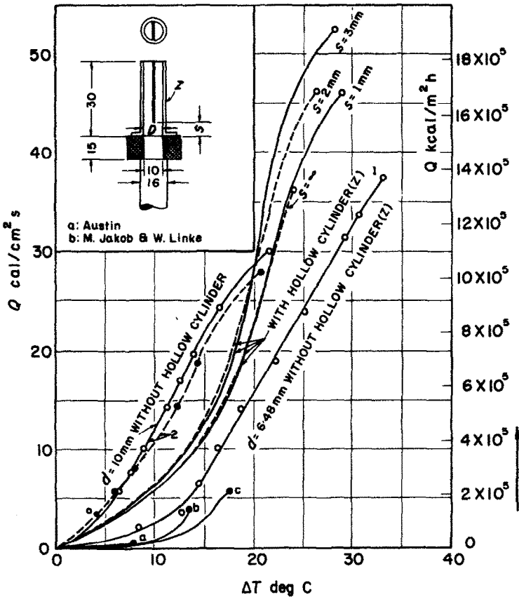
FIG. 1. \Delta T vs. Q curve; Water temperature = 100^{\circ}\text{C} .
