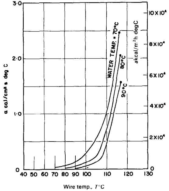
FIG. 13. \alpha curve for water temperature below 100^\circ\text{C} ; platinum wire, d = 0.19 \text{ mm} .
