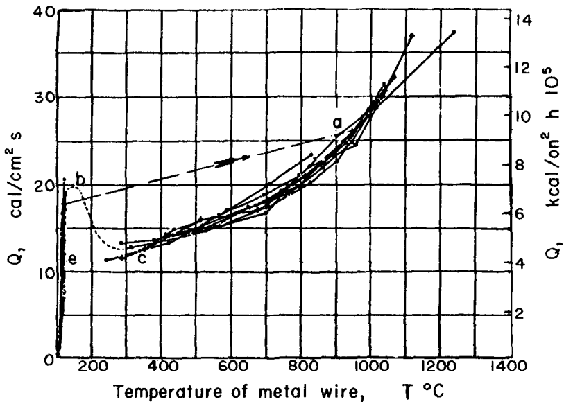
FIG. 14. The determination of Q_{\min} for the platinum wire of d = 0.14 \text{ mm} .
