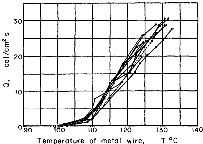
FIG. 6. Nickel wire, d = 0.40 mm (Nos. 1-10); water temperature = 100^{\circ}\text{C} .
