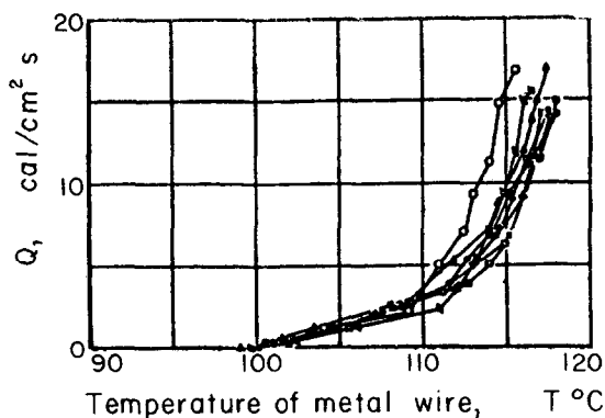
FIG. 4. Platinum wire, d = 0.14 mm; water temperature = 100°C.
