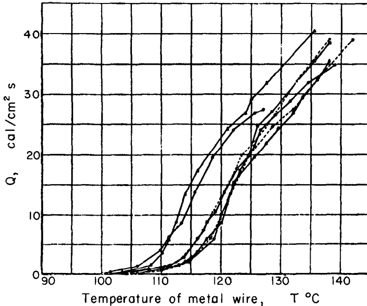
FIG. 8. Nichrome wire, d = 0.535 mm; water temperature = 100^\circ\text{C} .
