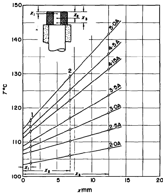
FIG. 16. Axial temperature distribution for the flat plate experiment.
