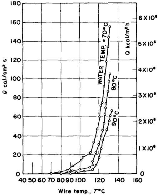
FIG. 12. Q curve for water temperature below 100^\circ\text{C} .
