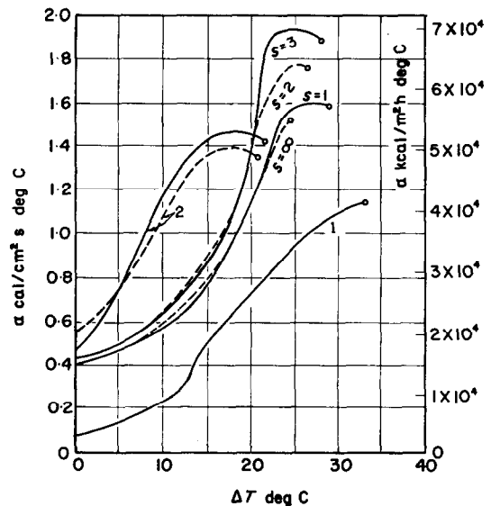
FIG. 17. \Delta T vs. \alpha curve; water temperature = 100^\circ\text{C} .
