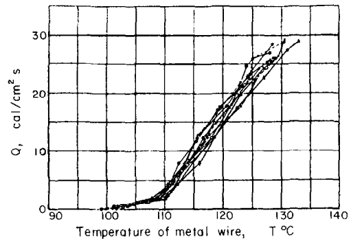
FIG. 7. Nickel wire, d = 0.40 mm (Nos. 11-20); water temperature = 100^{\circ}\text{C} .
