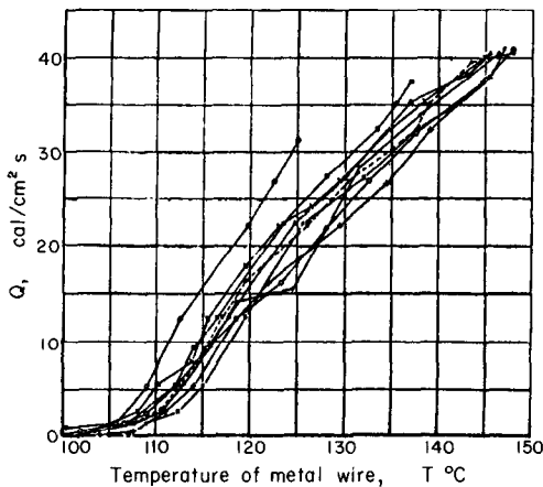
FIG. 9. Nichrome wire, d = 0.575 mm; water temperature = 100^\circ\text{C} .
