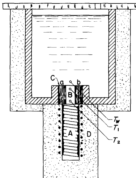
FIG. 15. Apparatus for the flat plate experiment.
