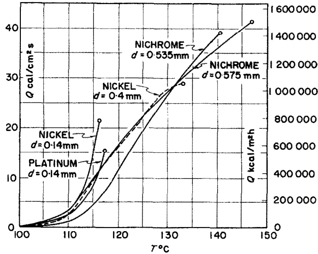
FIG. 10. Average value of Q for various metal wires; water temperature = 100^{\circ}\text{C} .
