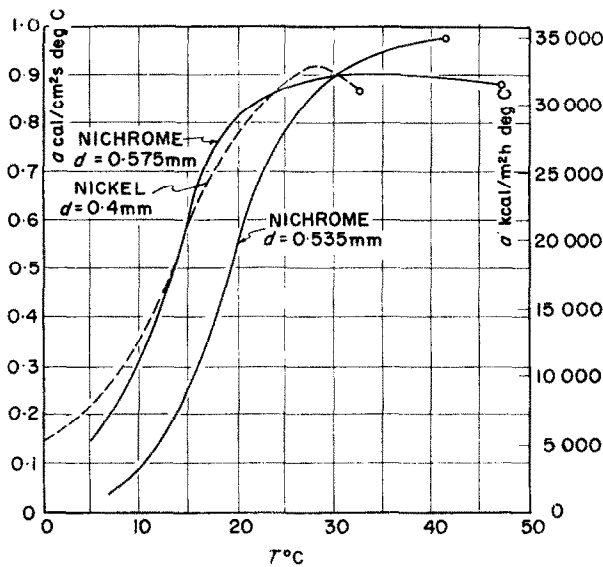
FIG. 11. Average value of \alpha for various metal wires; water temperature = 100^{\circ}\text{C} .
